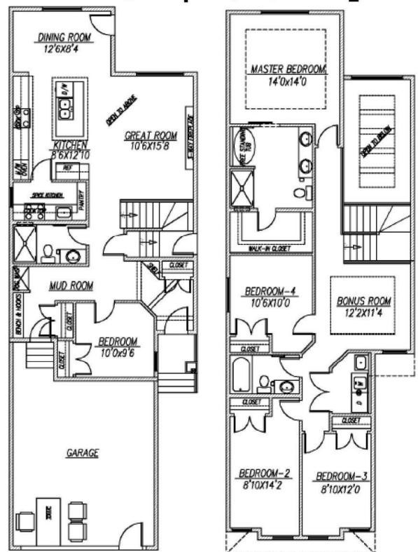
MAIN - 998 SQFT
